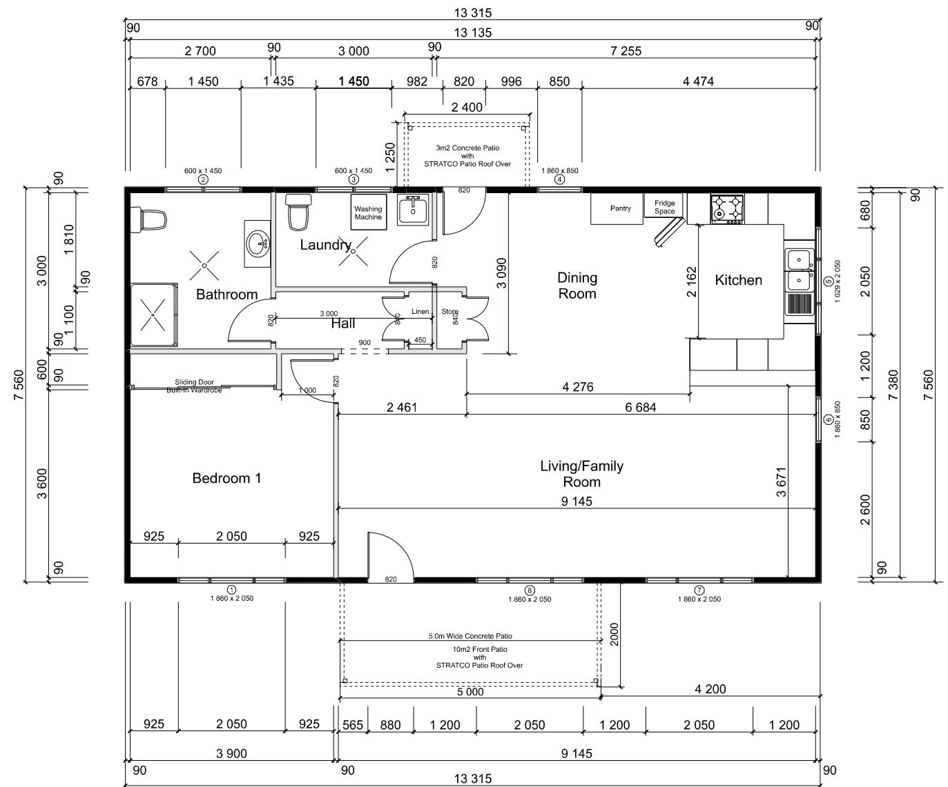
MODULAR BUILDING PLAN - 1 BED 93M2
