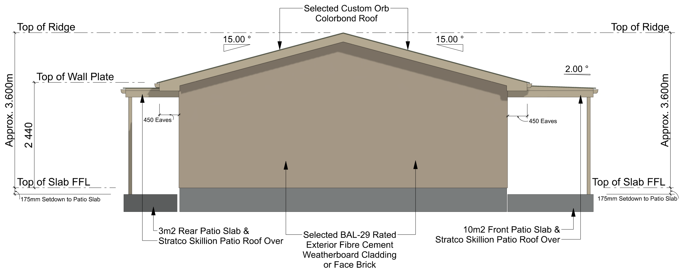
LEFT ELEVATION - 1 Bedroom - 93m2 - Residence SCALE: 1:50
