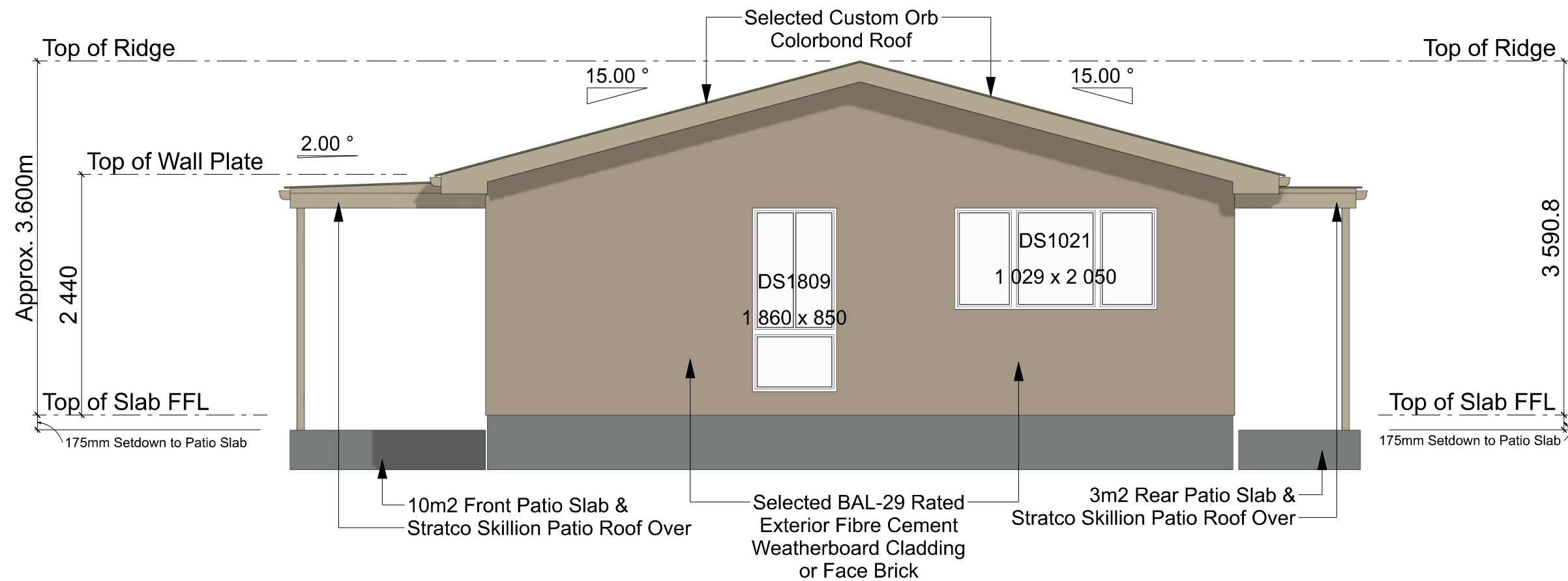
RIGHT ELEVATION - 1 Bedroom - 93m2 - Residence SCALE: 1:50
