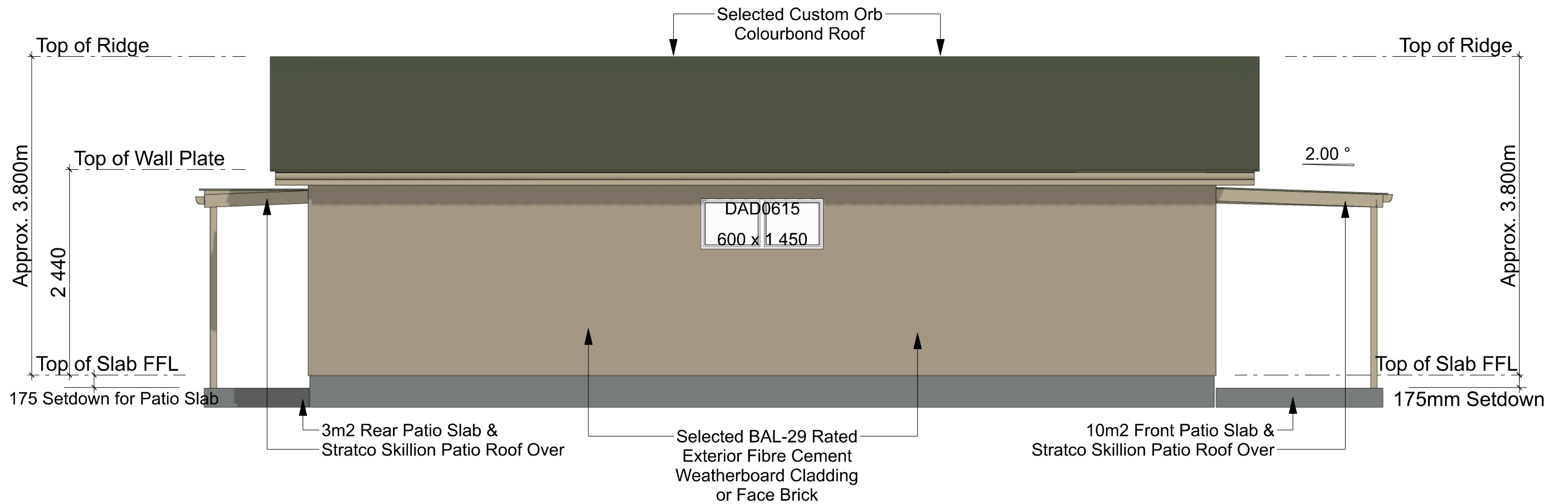
LEFT ELEVATION - 2 Bedroom - 93m2 - Residence SCALE: 1:50
