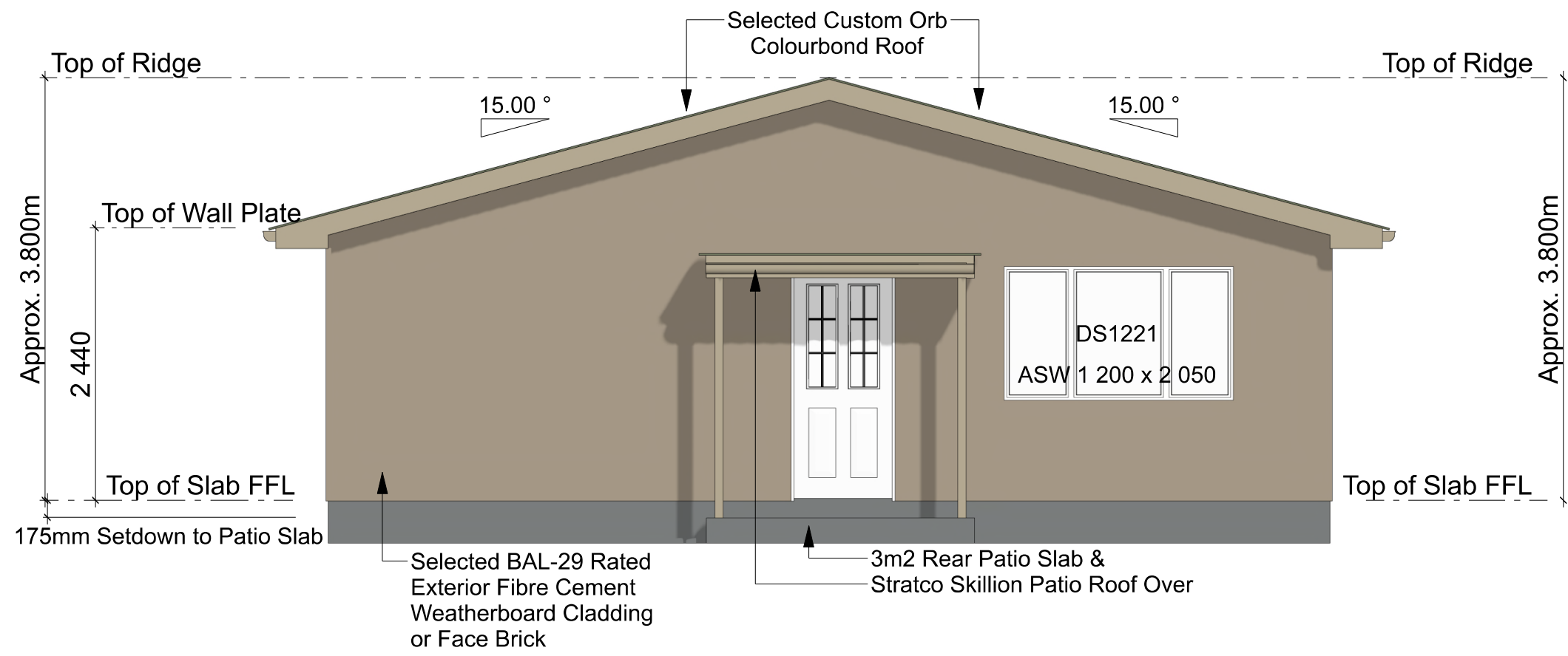
REAR ELEVATION - 2 Bedroom - 93m2 - Residence SCALE: 1:50
