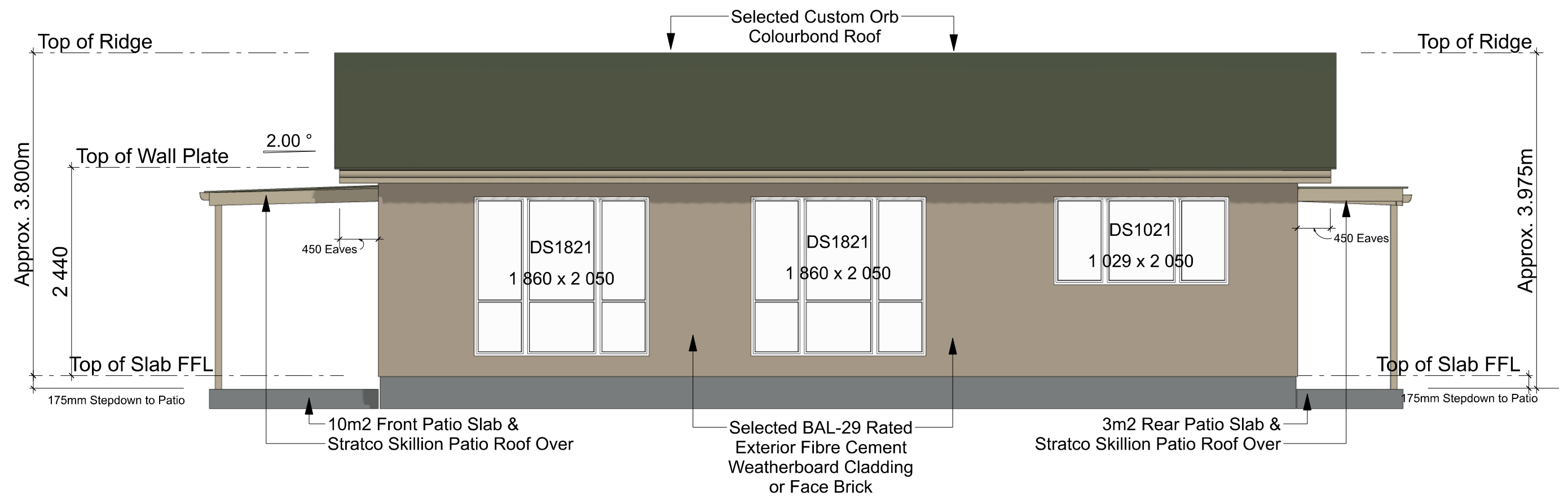
RIGHT ELEVATION - 2 Bedroom - 93m2 - Residence SCALE: 1:50
