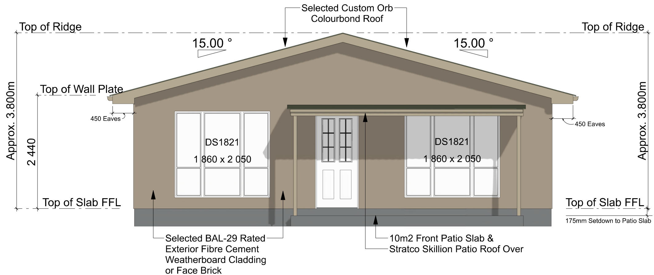
FRONT ELEVATION - 2 Bedroom - 93m2 - Residence SCALE: 1:50
