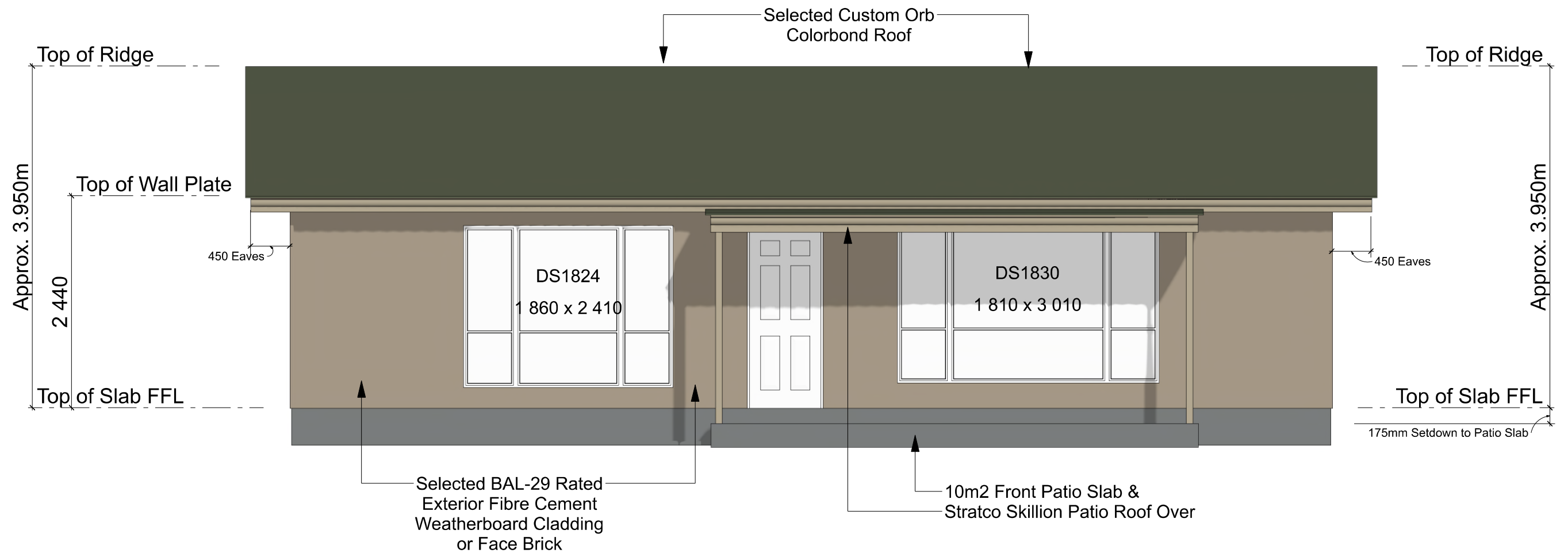
FRONT ELEVATION - 3 Bedroom - 119m2 - Residence with Ensuite SCALE: 1:50
