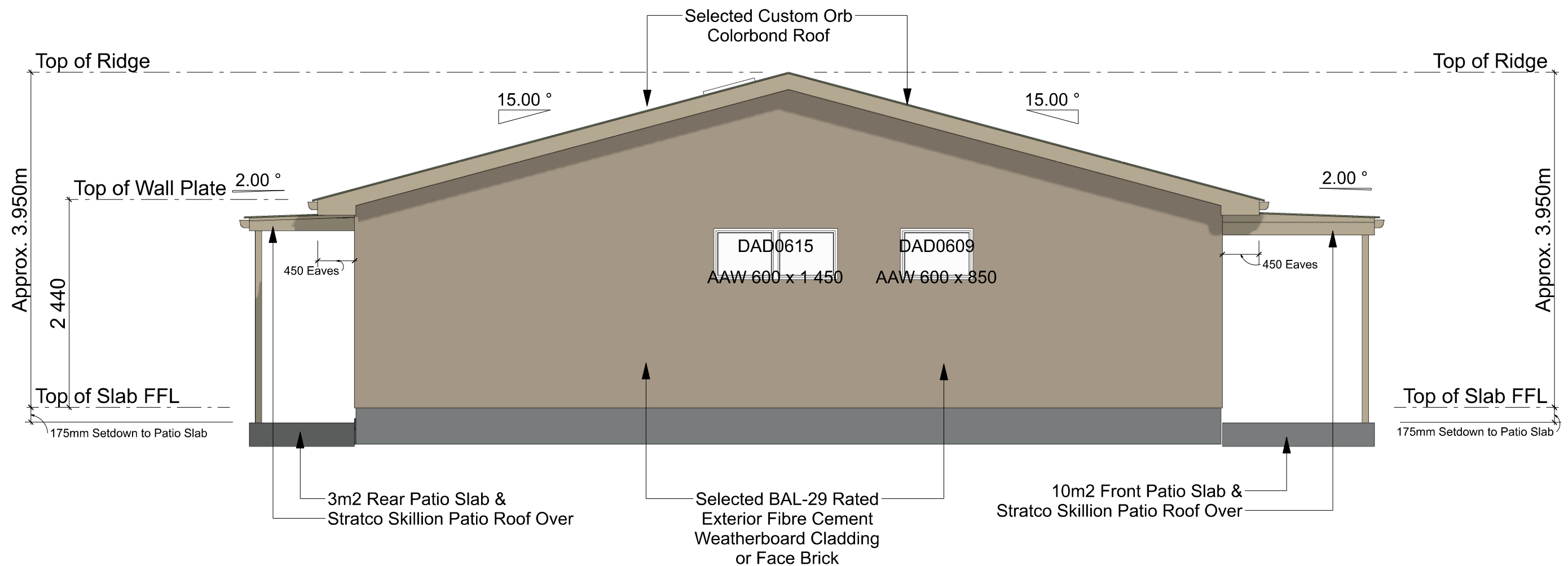
LEFT ELEVATION - 3 Bedroom - 119m2 - Residence with Ensuite SCALE: 1:50
