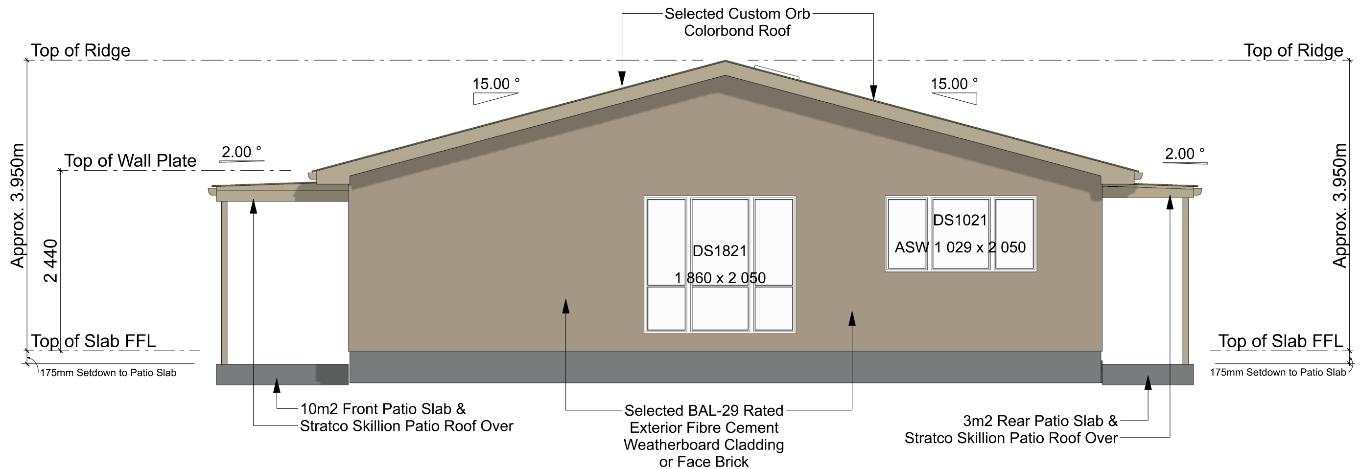
RIGHT ELEVATION - 3 Bedroom - 119m2 - Residence with Ensuite SCALE: 1:50
