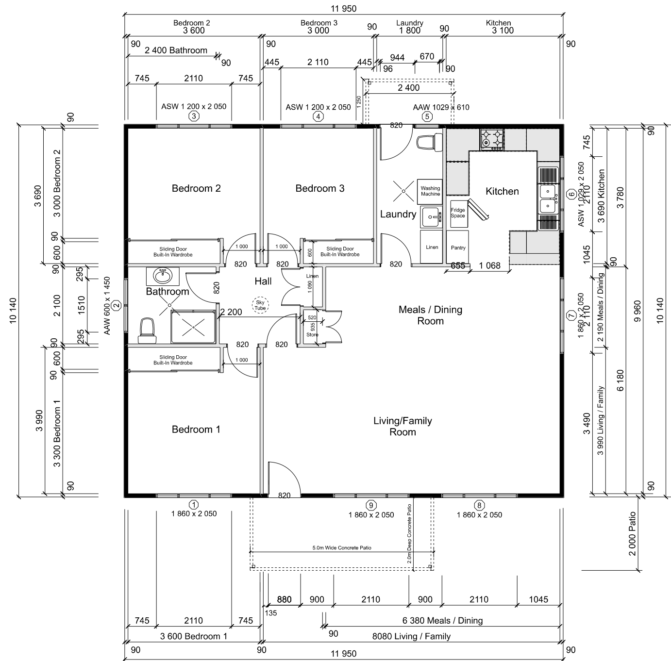
MODULAR BUILDING PLAN 3 BED - 119m2 Residence - No Ensuite
