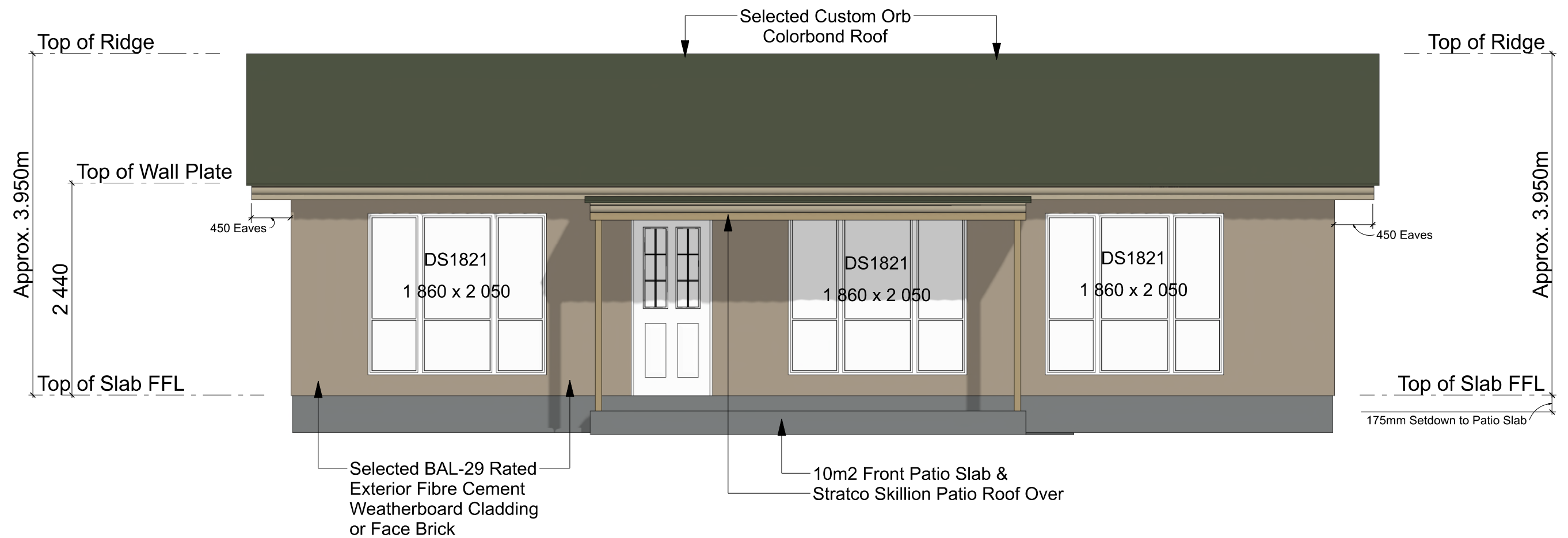
FRONT ELEVATION - 3 Bedroom - 119m2 - Residence SCALE: 1:50
