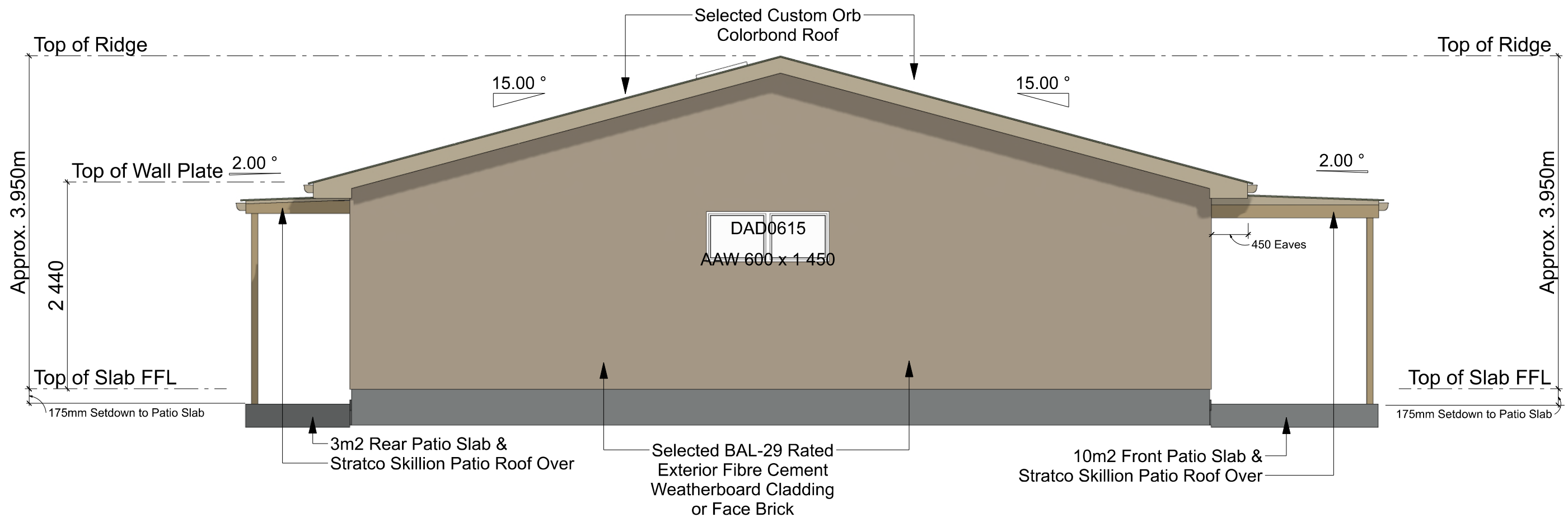
LEFT ELEVATION - 3 Bedroom - 119m2 - Residence SCALE: 1:50
