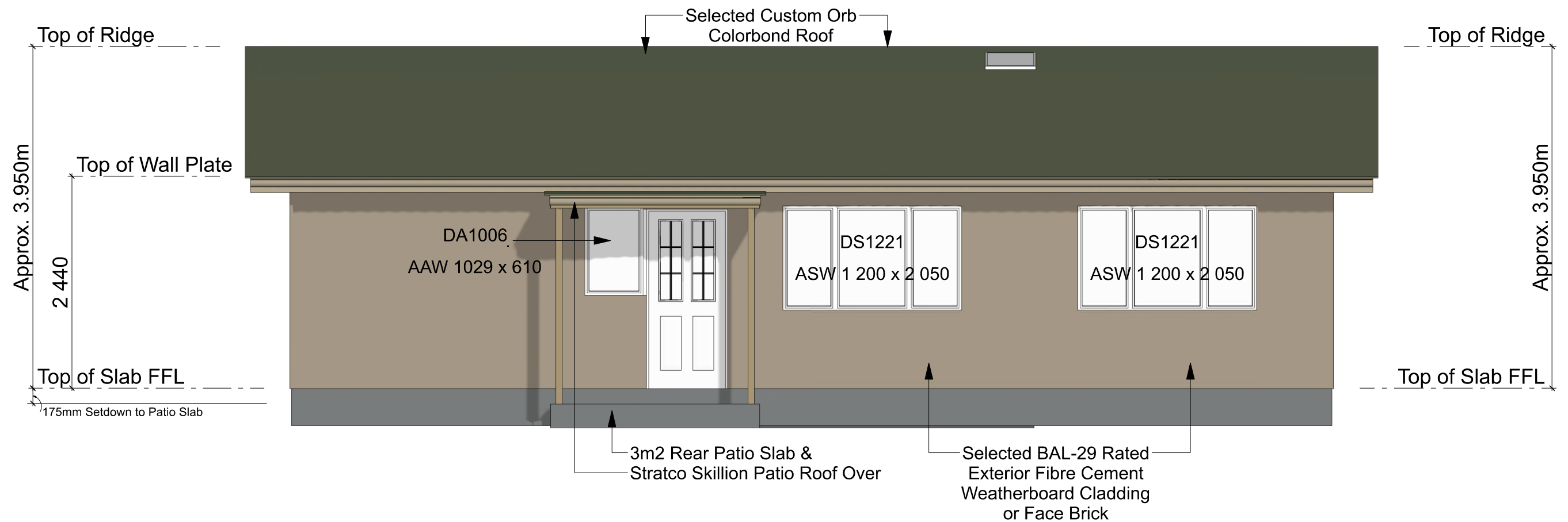
REAR ELEVATION - 3 Bedroom - 119m2 - Residence SCALE: 1:50
