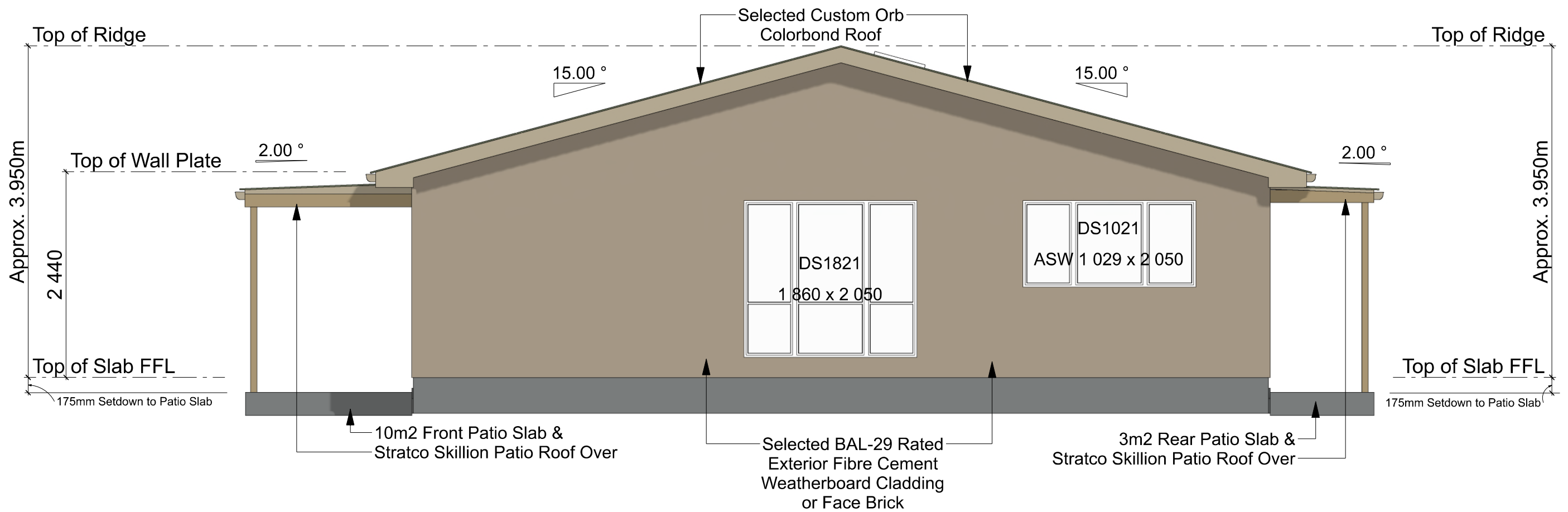
RIGHT ELEVATION - 3 Bedroom - 119m2 - Residence SCALE: 1:50
