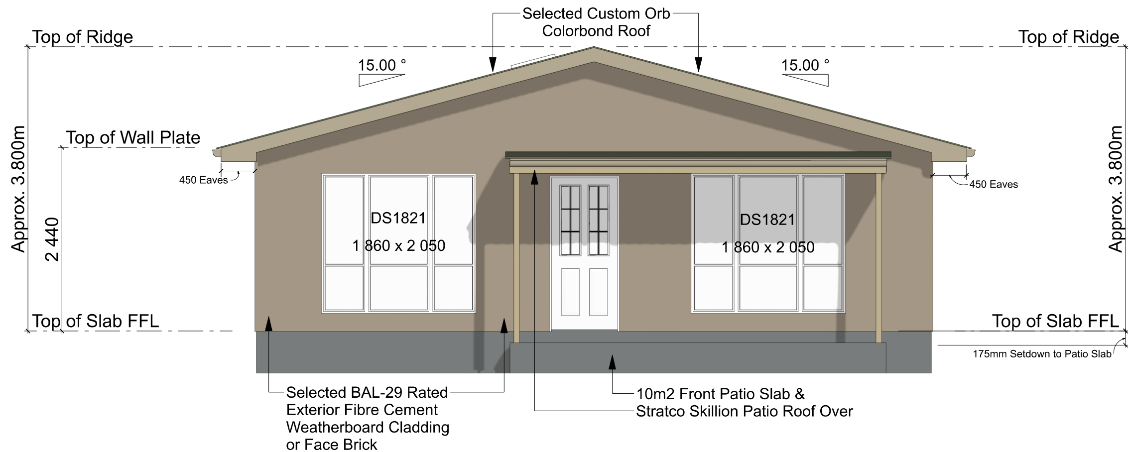
FRONT ELEVATION - 3 Bedroom - 93m2 - Residence SCALE: 1:50
