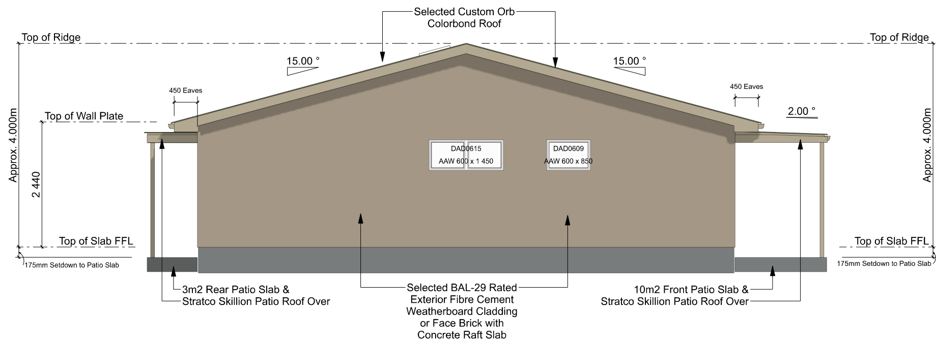
LEFT ELEVATION - 4 - 5 Bedroom - 192m2 - Residence with Ensuite SCALE: 1:75
