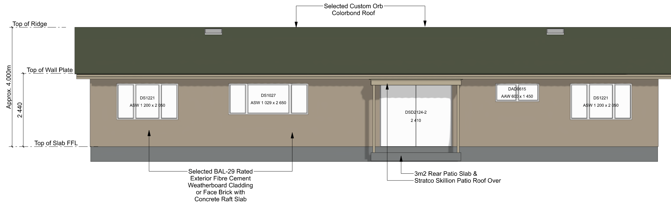
REAR ELEVATION - 4 - 5 Bedroom - 192m2 - Residence with Ensuite SCALE: 1:75
