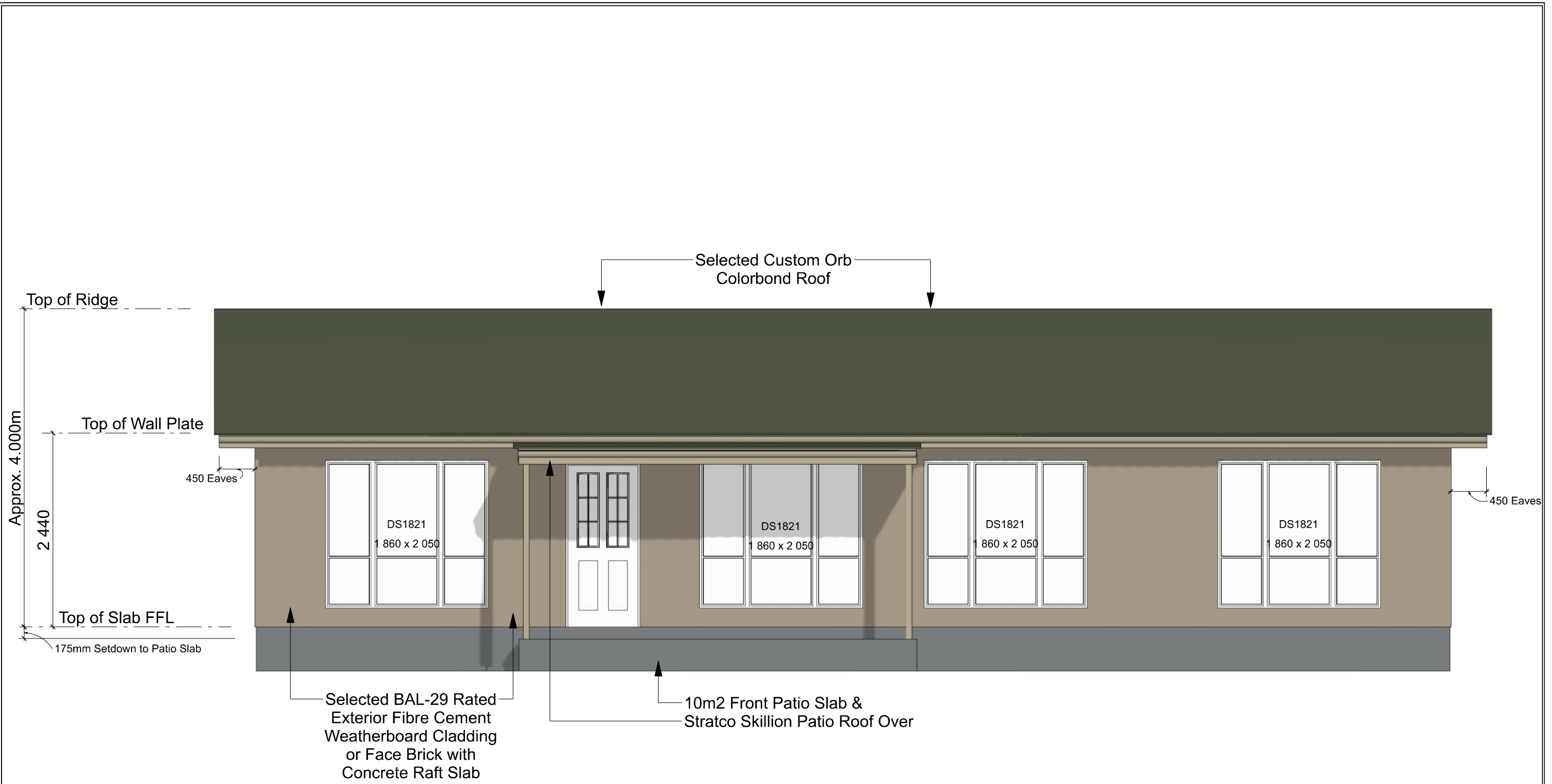
FRONT ELEVATION - 4 Bedroom - 155m2 - Residence SCALE: 1:50
