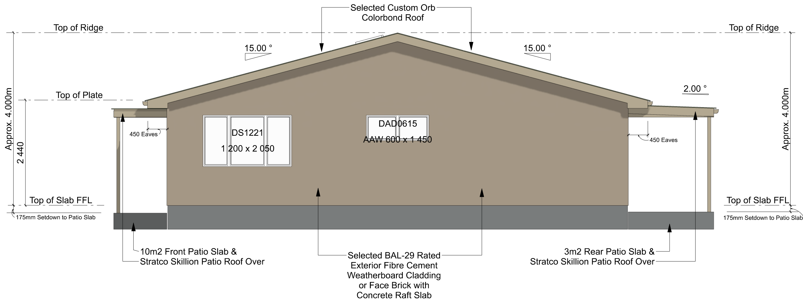
LEFT ELEVATION - 4 Bedroom - 155m2 - Residence SCALE: 1:50
