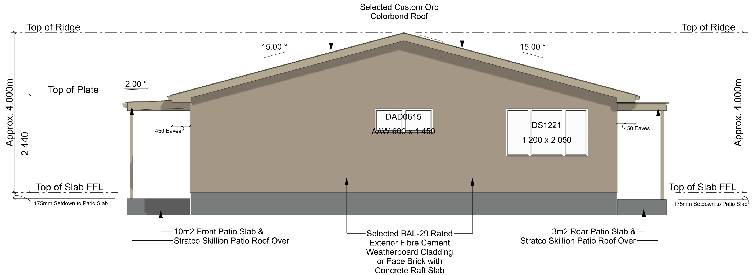
RIGHT ELEVATION - 4 Bedroom - 155m2 - Residence with Ensuite SCALE: 1:50
